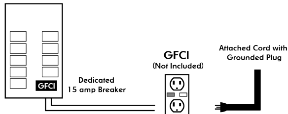
Main Power Supply
